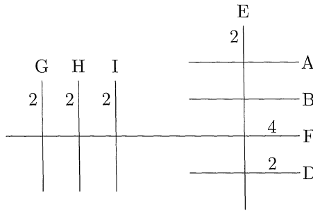
FIGURE 2. Special fiber of curve C_{63} over \mathbf{Z}_3
